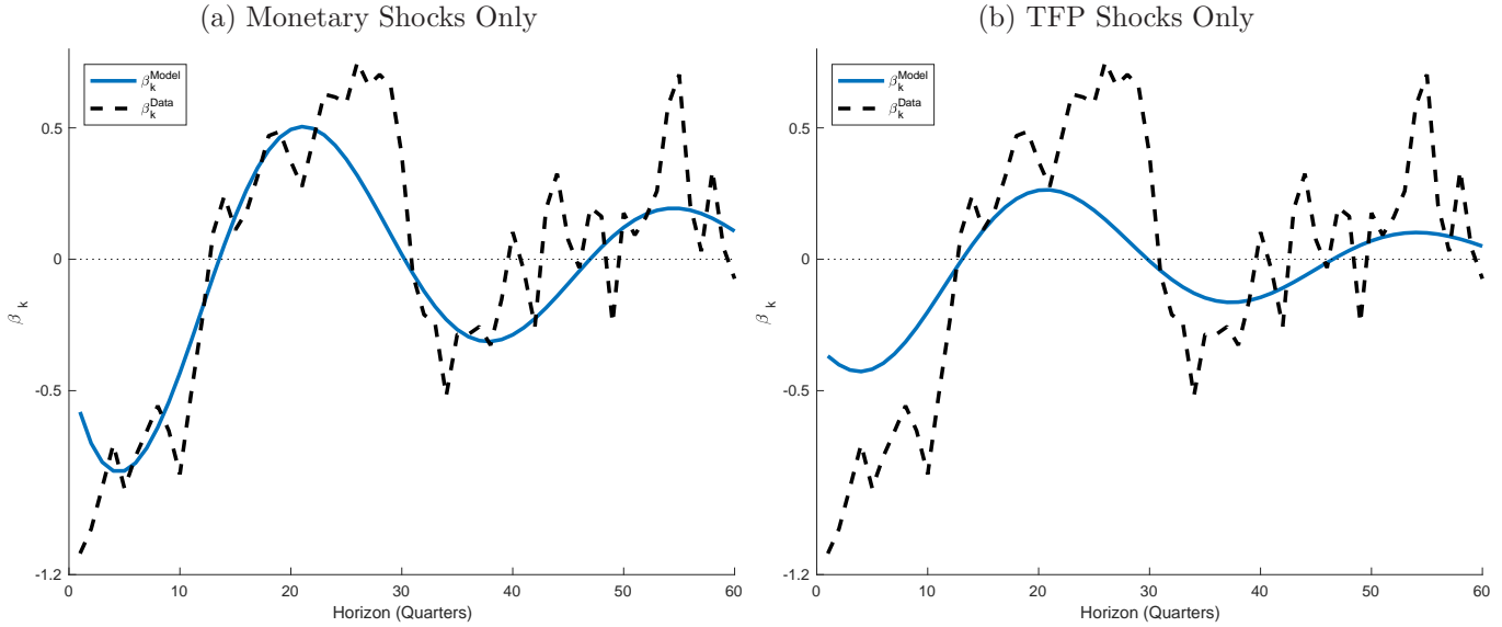
Figure 6: Regression Estimates, Model vs Data
