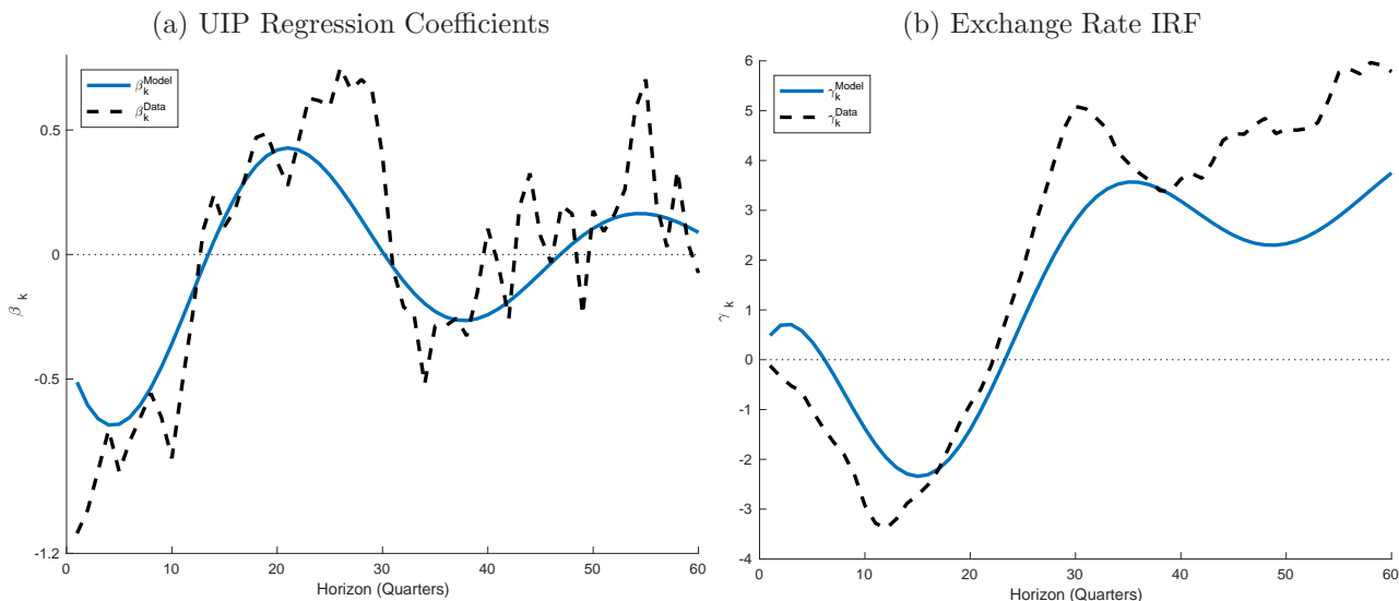
Figure 5: Regression Estimates, Model vs Data
