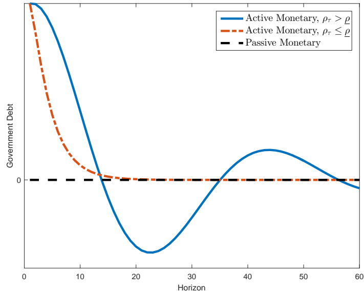
Figure 3: Equilibrium Debt Dynamics
