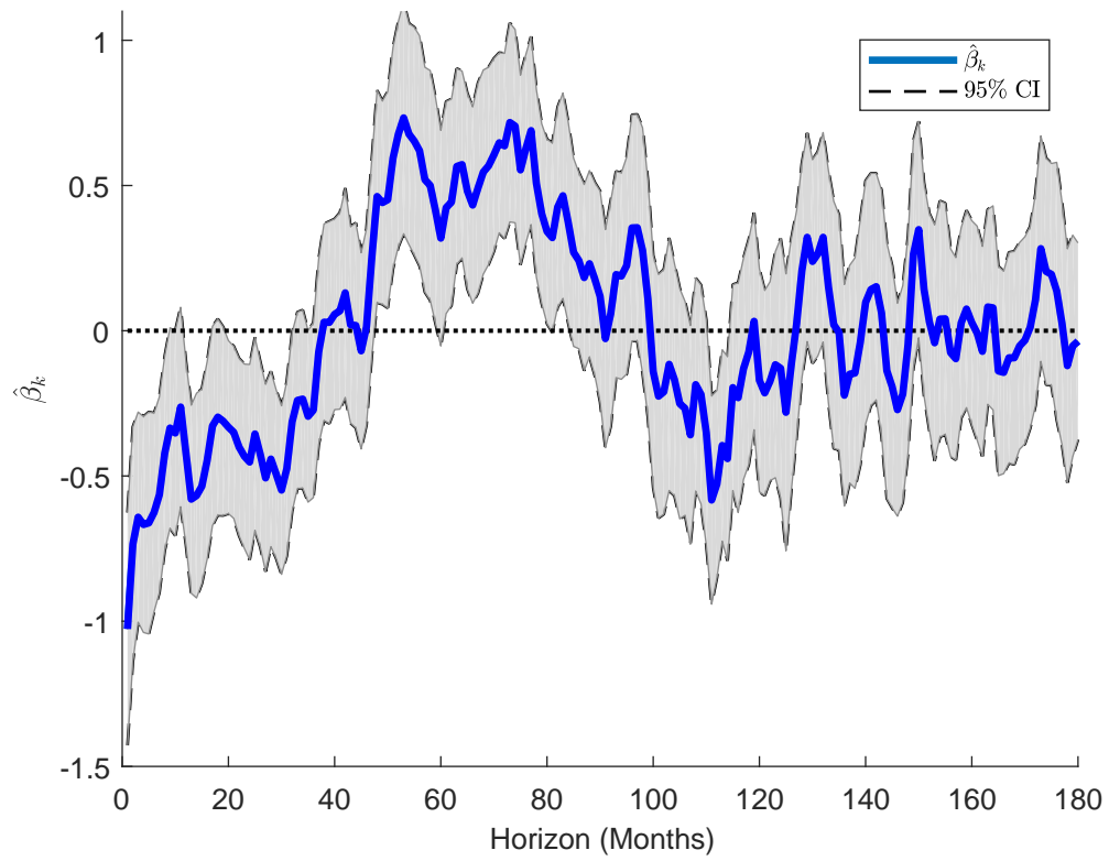
Figure B.1: UIP Violations Decomposition
