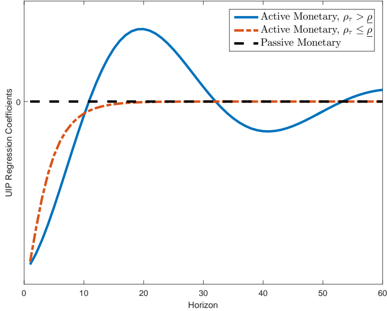
Figure 4: Model Implied UIP Regression Coefficients
